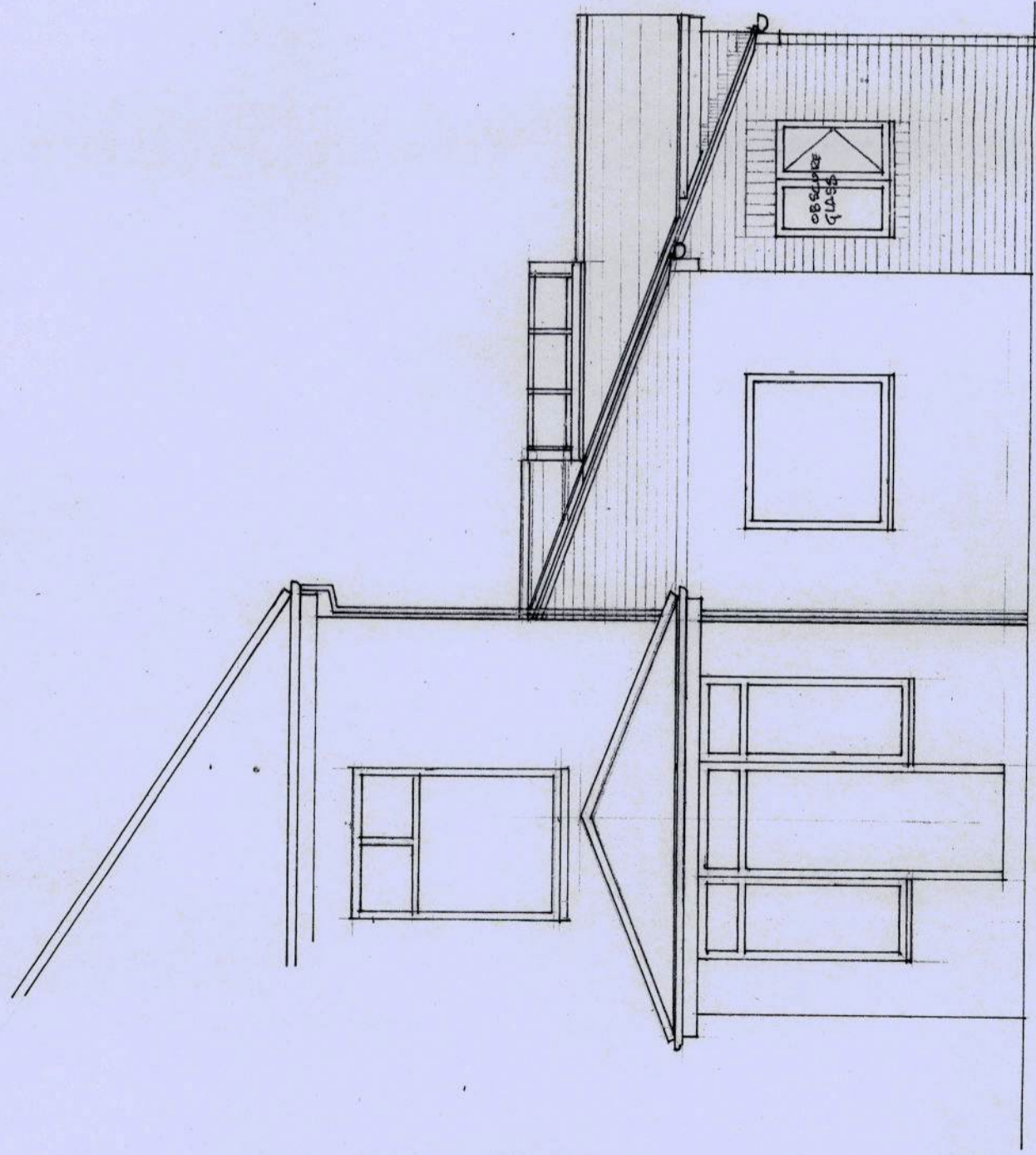
SOUTH ELEVATION
